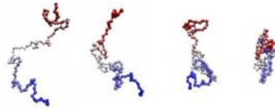
Protein folding
